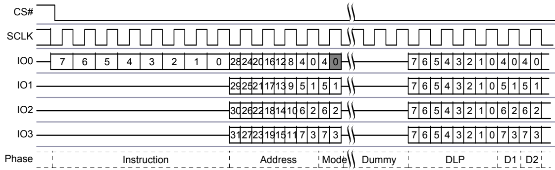
Figure 22. DDR Quad I/O Read Command
