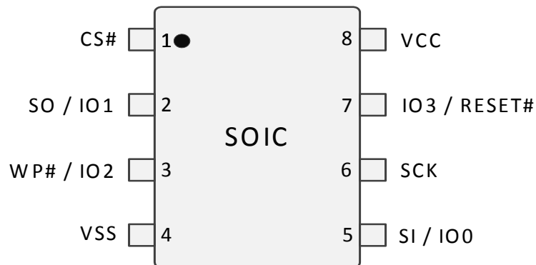
Figure 2. 8-Pin Plastic Small Outline Package (SOIC8)
