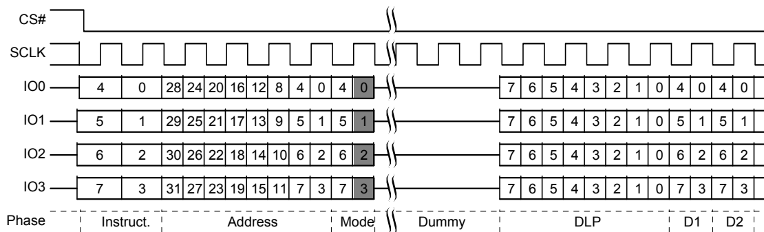
Figure 23. DDR Quad I/O Read Command QPI Mode
