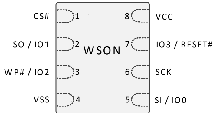
Figure 3. 8-Connector Package (WSO6 6x8) (WSO6 5x6), Top View
