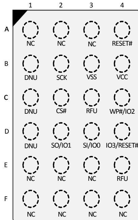
Figure 5. 24-Ball BGA, 4x6 Ball Footprint (FAC024), Top View
