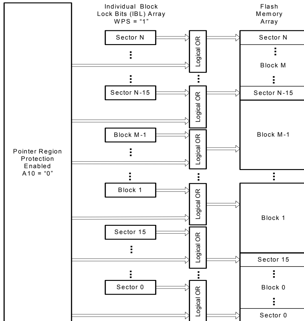
Figure 25. Individual Block Lock / Pointer Region Protection Control
