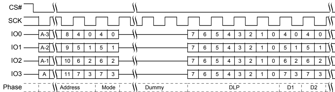
Figure 76. Continuous DDR Quad I/O Read Subsequent Access
