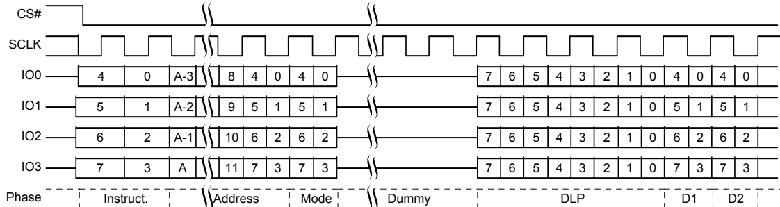
Figure 75. DDR Quad I/O Read Initial Access QPI Mode
