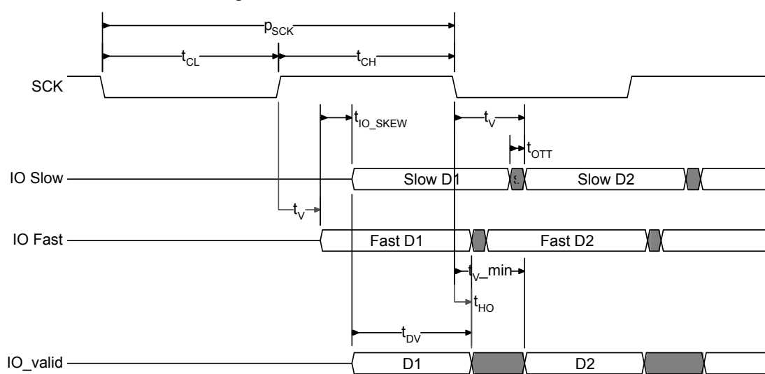
Figure 149. SPI DDR Data Valid Window
